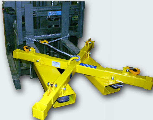
LIFTING FRAME LF 1000 F for fork-lifts
